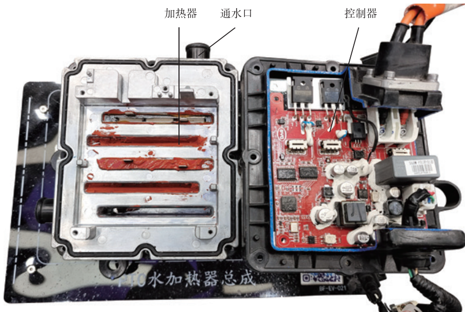
图 3-1-6 PTC
